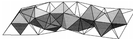
Fig. 15. Pearce's octahelix inscribed in a B-C structure.
