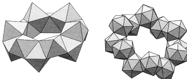
Fig. 18. A ring of twelve (slightly distorted) octahedra, generated by a roto-reflection; and the twelve inscribed icosahedra.
