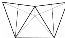
Fig. 21. Three tetrahedra. The ring of 96 tetrahedra is generated by twofold rotations about the face medians marked in the figure. Very slight deformation of the tetrahedra is necessary for exact closure of the ring, as explained in the text.
