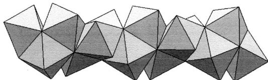
Fig. 17. An octahelix with steeper pitch.
