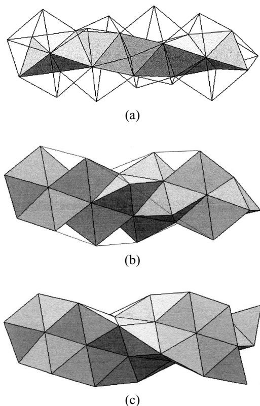
Fig. 6. Extension of the sphere packing. Sphere centers are at vertices of the tetrahedra. The additional tetrahedra are very nearly regular.
