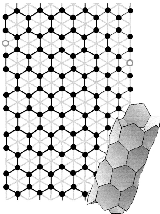
Fig. 9. The [1, 5, 6] nanotube derived from the (4, 7, 11) TPH.
