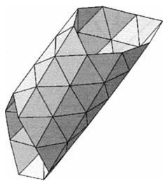
Fig. 2. The triangulated helical polyhedron (3, 5, 8) L .
