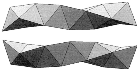
Fig. 4. The Boerdijk-Coxeter structures (1, 2, 3)R and (1, 2, 3)L.
