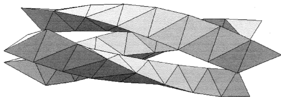
Fig. 11. General view of the three outer B-C structures of the collagen model proposed by Sadoc and Rivier. The polypeptide chains correspond to the type {2} helices of these structures. Other edges and edges of the central undeformed B-C structure (omitted for clarity) correspond to hydrogen bonds.
